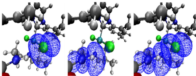
Fig. 3 NBO orbitals for precatalyst A for system 1 involved in the \text{NH}\cdots\text{Cl} interaction: LP (left), \text{BD}^* (middle) and overlap of the latter orbitals (right), see ESI† for further details.
