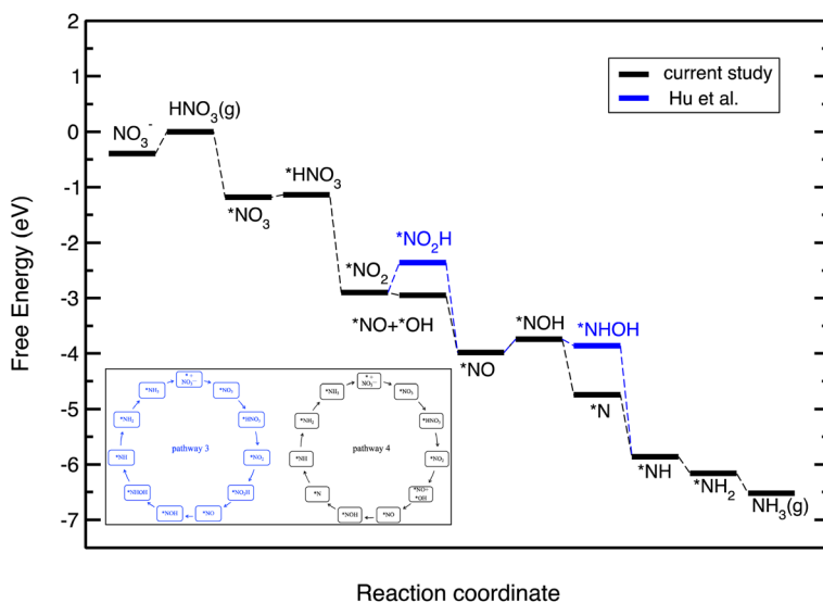
Fig. 5 Free energy diagrams for the \text{NO}_3\text{RR} on \text{Cu}(111) . The black line denotes the constructed free energy diagram in the present study. The blue line shows the free energy diagram suggested by Hu et al. 50 The inset shows the reaction pathway for the \text{NO}_3\text{RR} to ammonia on \text{Cu}(111) reported by Hu et al. (pathway 3 in Fig. 3) as well as the one obtained in the present study (pathway 4).
