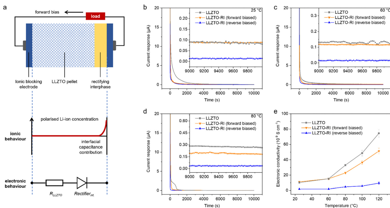
Fig. 3 (a) Schematic diagram of the ionic behaviour and electronic behaviour for the LLZTO-RI pellet with two ionic blocking electrodes. (b–d) Chronoamperometry curves under a constant direct current polarisation of 1 V. Inset: current response at the equilibrium state. (e) Electronic conductivities at different temperatures. Error bars represent the variance of current fluctuations during the steady states.
