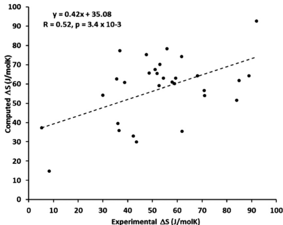
Fig. 3 Scatter plot of the experimental and computed entropy changes during spin crossover for 30 complexes studied by Kepp with the trend line showing relatively poor linear correlation. Reprinted with permission from ref. 17, Copyright (2016) American Chemical Society.
