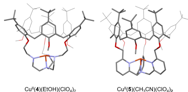
Fig. 5 Views of the XRD structures of \text{Cu}^{\text{II}} complexes based on the 4 and 5 calix[6]arene-based ligands. Counter ions and bounded molecules of solvent (EtOH and \text{CH}_3\text{CN} , respectively) have been omitted for clarity.
