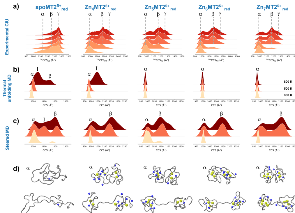
Fig. 4 Collision cross section (CCS) profiles for the quadrupole-selected apoMT2 5+ red and Zn 4-7 MT2 5+ red species under different collisional activation energies (a). Gaussian kernel density estimate (KDE) for 300 K, 500 K and 800 K slices from thermal unfolding simulations (b). Gaussian KDE for steered MD simulations with 10, 25 and 50 kcal mol -1 nm -2 force constants (c). Representative snapshots for the conformations from each protein species labeled as in the Gaussian KDE (d). Yellow and blue spheres represent Zn 2+ and Na + , respectively, and the protein backbone is shown in grey.
