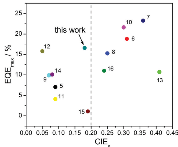
Fig. 7 Summary of \text{EQE}_{\text{max}} and \text{CIE}_y values of recently reported SP-OLEDs. The reference numbers are presented next to the relevant data points.
