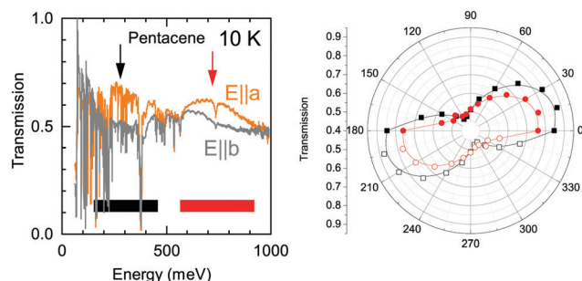
Fig. 6 Transmission spectra for two perpendicular polarizations measured at T = 10 K. The electronic background centered around 200–300 meV and 750 meV shows a clear polarization dependence with a maximum and minimum aligned with the optical a - and b -axes. The angular dependence is presented in the right panel where the open symbols denote the symmetrized part of the polarization dependent measurements. Red and the black symbols belong to the peak pointed with the red and black arrows in the left panel, respectively.
