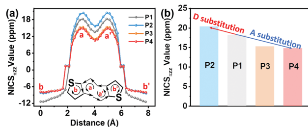
Fig. 4 The NICS-XY scans (a) and pentadiene core NICS values (b) of the indicated compounds involved in this study.
