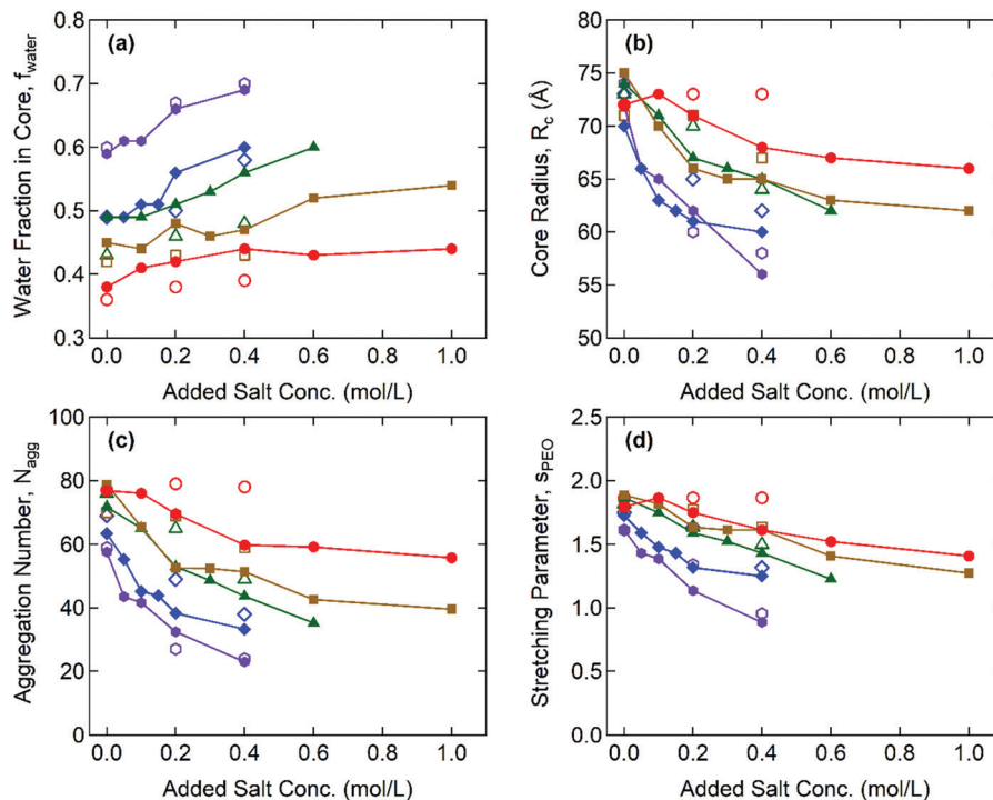
Fig. 4 SAXS (closed symbols) and SANS (open symbols) fit results from G_{0.0} + S (purple/hexagons), G_{0.32} + S (blue/diamonds), G_{0.49} + S (green/triangles), G_{0.76} + S (brown/squares), and G_{0.95} + S (red/circles) hydrogels as functions of the added salt concentration. (a) Water fraction in the coacervate core, (b) core radius, (c) aggregation number, and (d) dimensionless parameter of the PEO chain stretching.
