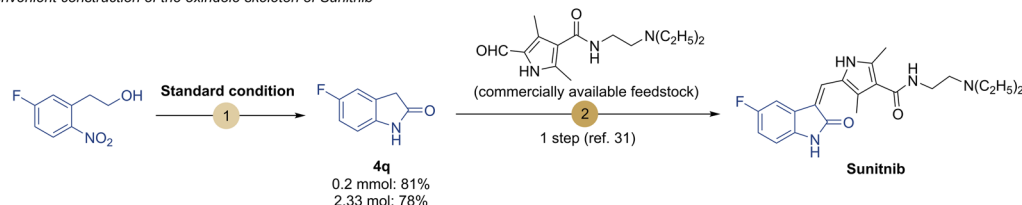
Scheme 4 Synthetic applications.
