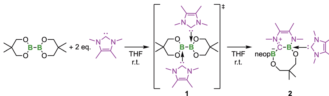
Scheme 2 Reaction of B_2neop_2 with two equivalents of Me_2Im^{Me} at room temperature forming the ring expanded product RER- B_2neop_2 -( Me_2Im^{Me} ) 2 2 with the bis-NHC adduct ( Me_2Im^{Me} ) 2 · B_2neop_2 1 as an intermediate.
