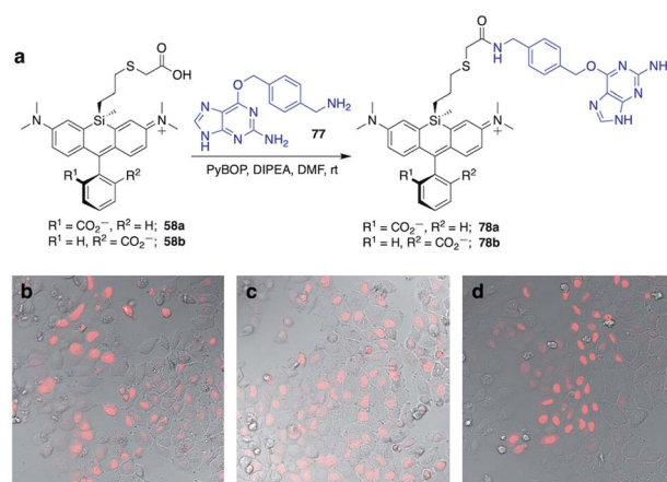
Fig. 4 Synthesis of Si-bridge dyes 78a–b and their use for live-cell imaging of HeLa cells transfected with pSNAPf-H2B. (a) Synthesis of 78a–b by the reaction of 58a–b with O 6 -benzylguanidine coupling partner 77 ; (b–d) Overlay of dye fluorescence and DIC for cells treated with 3 \mu\text{M} (b) SNAP-Cell 647-SiR, (c) 78a , or (d) 78b . Scale bar is 20 \mu\text{m} .
