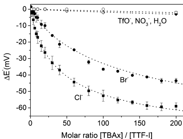
Fig. 25 Cathodic voltammetric perturbations of the first oxidative couple of iodo-TTF 23XB in DMF upon addition of various anions. Reproduced from ref. 138 with permission from the PCCP Owner Societies.
