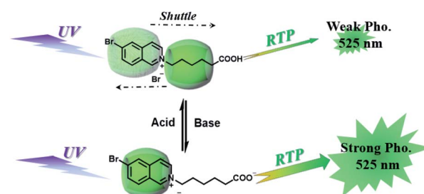
Fig. 5 Schematic illustration of the construction of a pH-controlled molecular shuttle in aqueous solution based on CB[7] and the 6-bromoisoquinoline derivative.
