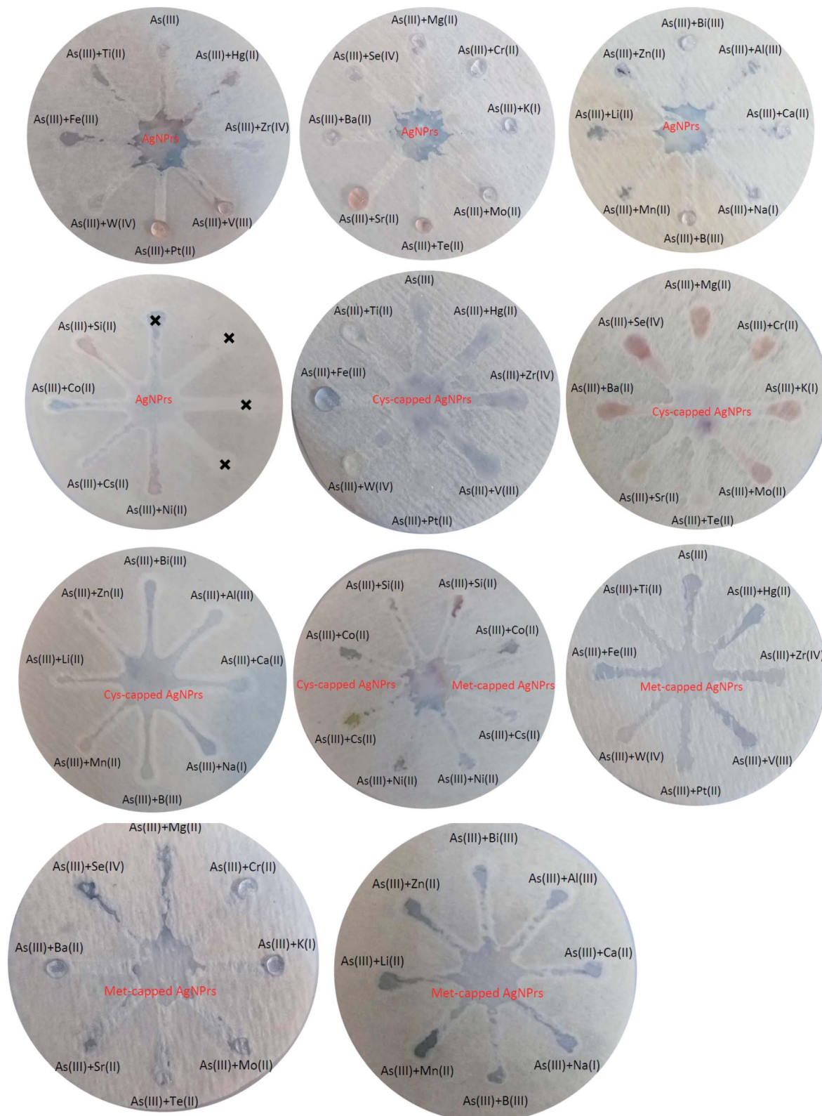
Fig. 4 Selectivity analysis of sensing probes for identification of As(III) in the presence of other metal ions using μPADs.
