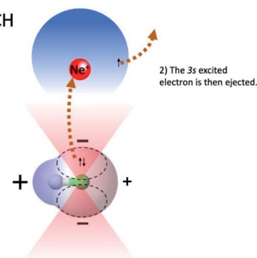
Fig. 5 Schematization of atomic and molecular orbitals of reagents and perpendicular configuration of the precursor state promoting the formation of HX^+ ion in the ground ( X^2\Pi ) electronic state. Most relevant electronic rearrangements involved in the direct mechanism are indicated in the figure, where also the shape of acceptance angular cones, where reaction is effectively stimulated, is also depicted.
