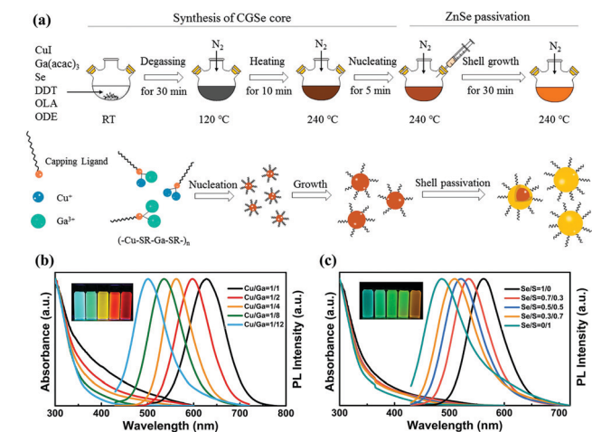
Fig. 4 (a) Schematic illustration of the synthetic procedures of CuGaSe/ZnSe core/shell QDs via a heating-up method. UV-vis absorption (left), PL spectra (right, \lambda_{\text{ex}} = 405 nm) and digital photograph of samples under the radiation of 365 nm UV illumination (inset) of (b) CuGaSe/ZnSe and (c) CuGaSe x S 1-x /ZnSe QDs prepared under various Cu/Ga and Se/S precursor molar ratios, respectively. Reproduced with permission. 40 Copyright 2018 Elsevier B.V. All rights reserved.
