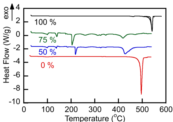
Fig. 3 DSC melting endotherms on 10\text{ °C min}^{-1} heating of the carbonate ( \text{Li}_{1.24}\text{K}_{0.76}\text{CO}_3 ) and borate ( \text{Li}_{1.5}\text{Na}_{1.5}\text{BO}_3 ) and their blends in nitrogen atmosphere. Numbers indicate nominal initial content of borate (mol%) in the blends. Endotherms were shifted along the heat flow axis for the presentation clarity, while preserving the original scale. Solid and dashed lines represent endotherms obtained using a Discovery DSC 250 (sealed pans) and Q600 (open to nitrogen atmosphere), respectively.
