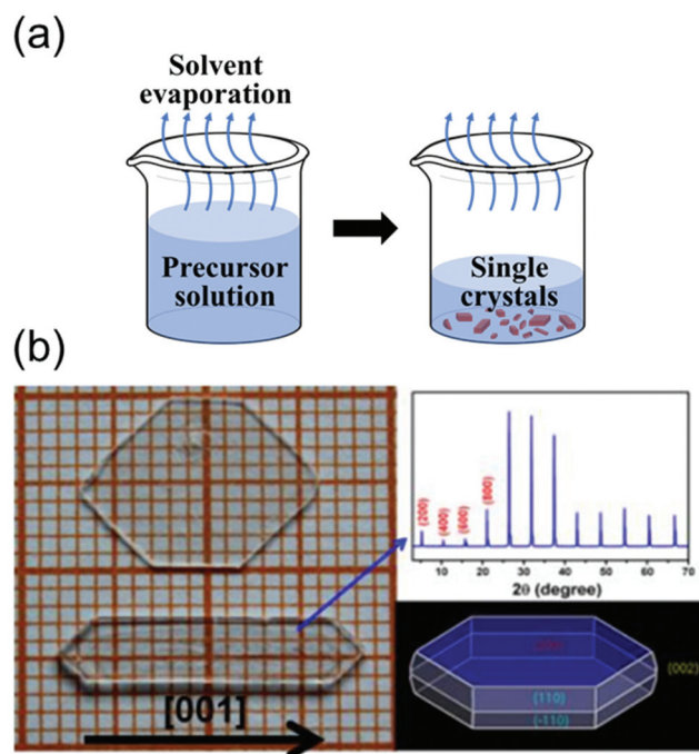
Fig. 5 (a) Schematics of the solvent evaporation crystallization method. (b) Image of two large single crystals of \text{BA}_2\text{PbCl}_4 , and the simulated morphology obtained using Material Studio. Photographs indicating the size of the \text{MAPbCl}_3 single crystal as well as the (100) crystallographic plane. The single crystals were prepared at different temperatures. Reproduced with permission. 69 Copyright 2015, Springer Nature.
