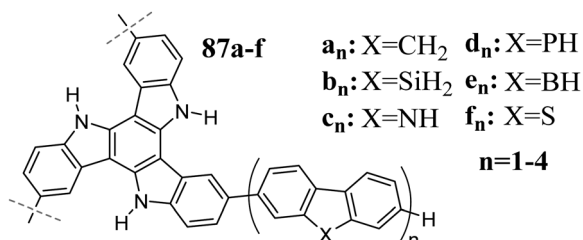
Scheme 30 Tri(oligoheterofluorene) 5,10,15-triazatruxenes.
