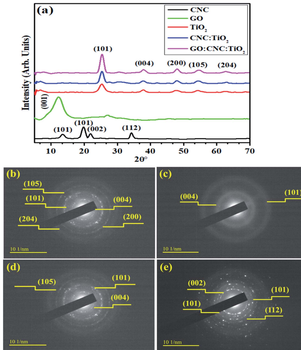
Fig. 2 (a) XRD patterns and (b–e) SAED patterns of CNC, \text{TiO}_2 , \text{CNC/TiO}_2 and \text{GO/CNC} -doped \text{TiO}_2 QDs, respectively.
