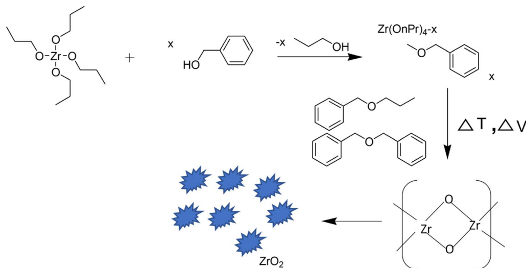
Fig. 3 Reaction mechanism of the nonaqueous synthesis of ZrO 2 nanoparticles. 28
