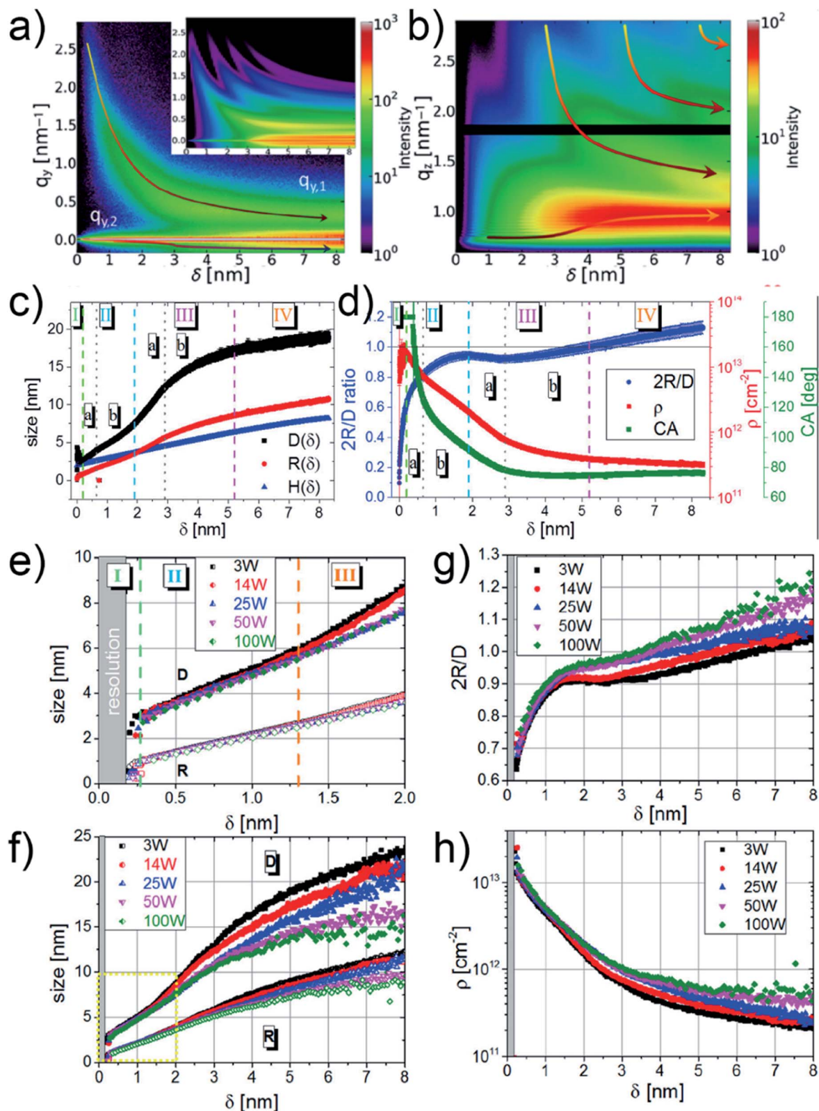
Fig. 5 Mappings of (a) out-of-plane line cuts (at the PS Yoneda peak of q_z = 0.69 nm ^{-1} ) and (b) off-detector line cuts (at q_z = 0 nm ^{-1} , 0.187 nm ^{-1} < q_y < 2.852 nm ^{-1} ) of 2D GISAXS data versus deposited Au effective thickness. (c) Evolution of inter-cluster distance D (black), cluster radius R (red), and cluster height H (blue). (d) Evolution of cluster diameter over distance ratio 2R/D (blue), cluster density \rho (red), and contact angle CA (green). Reproduced with permission. 49 Copyright 2015 American Chemical Society. Evolution of inter-cluster distance D and cluster radius R at different sputter powers of 3 W (black), 14 W (red), 25 W (blue), 50 W (magenta), and 100 W (green) in the (e) first 2 nm and (f) first 8 nm effective thickness, respectively. Evolution of (g) cluster diameter over distance ratio 2R/D and (h) cluster density \rho at different sputter powers of 3 W (black), 14 W (red), 25 W (blue), 50 W (magenta), and 100 W (green). Reproduced with permission. 51 Copyright 2017 American Chemical Society.
