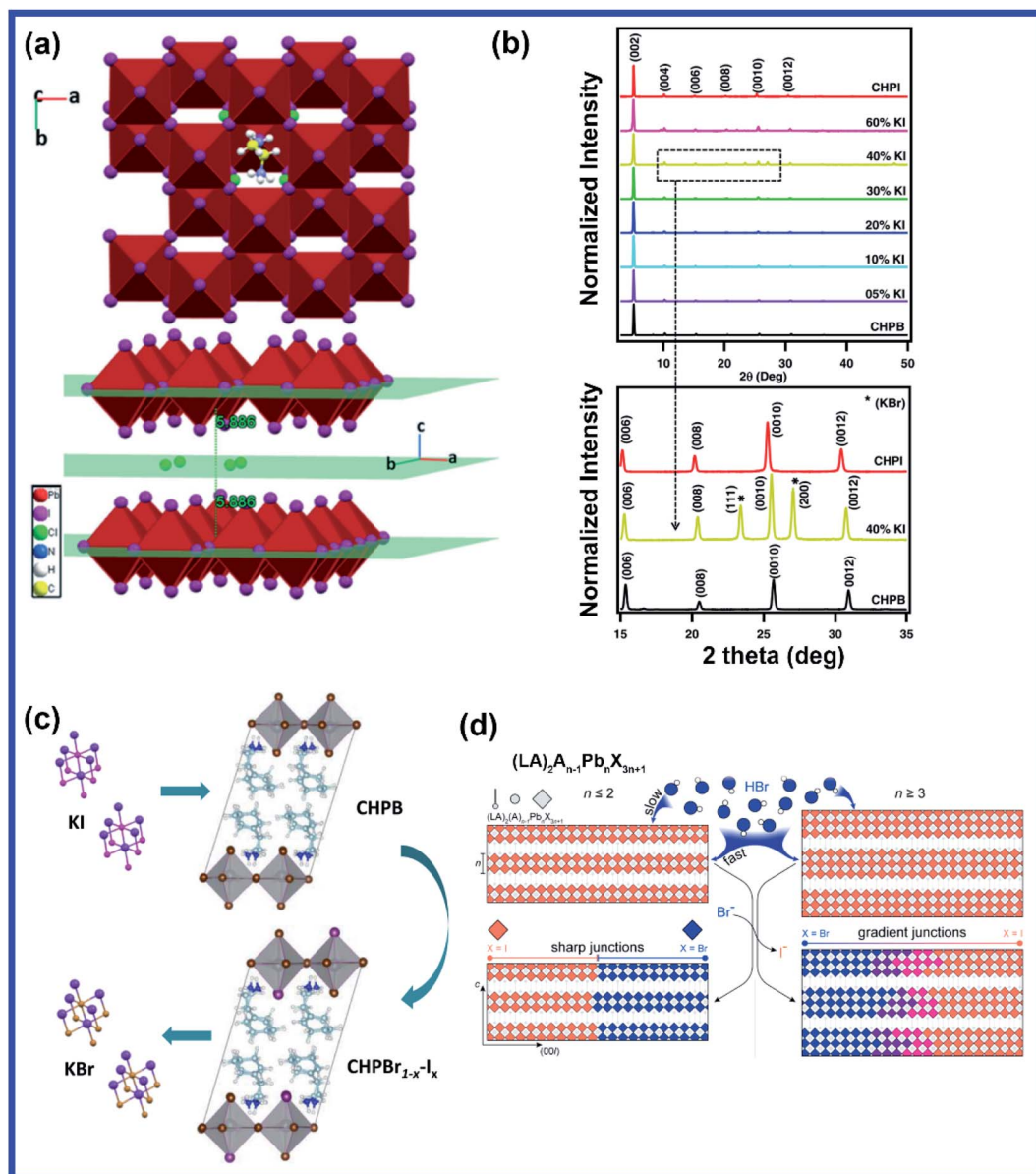
Fig. 6 (a) Schematic diagram of \text{EDPbI}_4 crystal and accommodation of chloride ions in the ab -plane between the inorganic sheet layers. Reprinted with permission from ref. 93. Copyright 2020, Royal Society of Chemistry. (b) XRD spectra of the mixed halide 2D perovskite with different vol% of KI and (c) schematic presentation of the formation of the mixed halide perovskite with the inclusion of KI and the byproduct. Reprinted with permission from ref. 95. Copyright 2020, American Chemical Society. (d) Schematic illustration depicting the different outcomes of vapor–solid anion exchange in lead iodide perovskites using HBr vapor depending on the layer thickness. Reprinted with permission from ref. 101. Copyright 2021, American Chemical Society.
