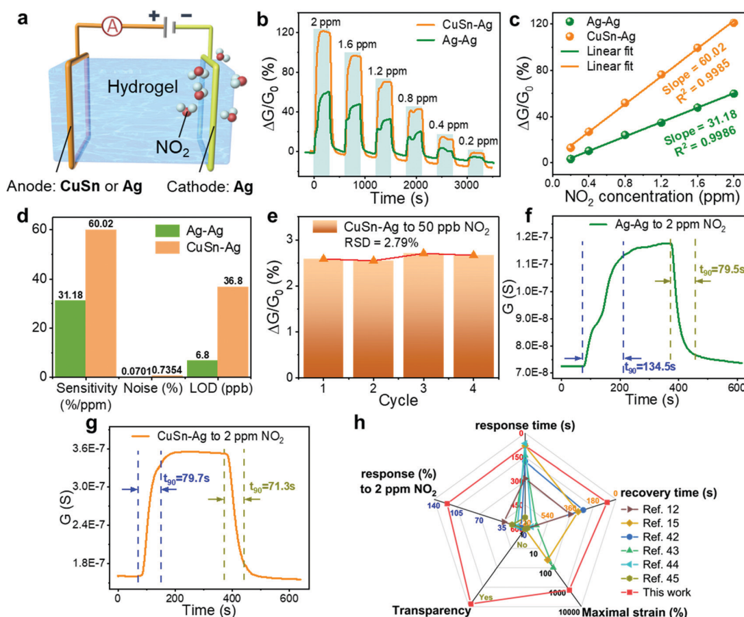
Fig. 4 \text{NO}_2 sensing properties of the DN hydrogel-based sensor. (a) Schematic diagram showing the device structure of the hydrogel-based sensor. (b) Dynamic response curves of the Ag-Ag and CuSn-Ag sensors to a series of \text{NO}_2 concentrations. (c) Linearly fitted response versus \text{NO}_2 concentration, from which the sensitivities were derived. (d) The comparison of the Ag-Ag and CuSn-Ag sensors in terms of the sensitivity, noise and LOD. (e) Repetitive sensing tests of the CuSn-Ag sensor toward 50 ppb \text{NO}_2 . (f) and (g) Analyses of the response and recovery times of the Ag-Ag and CuSn-Ag sensors to 2 ppm \text{NO}_2 . (h) The performance comparison of different flexible \text{NO}_2 sensors.
