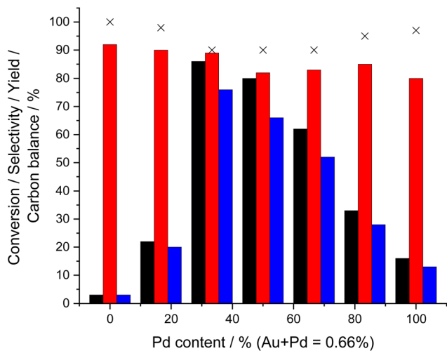
Fig. 2 The effect of Au: Pd ratio on catalytic activity towards the ammoxidation of cyclohexanone via in situ \text{H}_2\text{O}_2 production. Ammoxidation reaction conditions: cyclohexanone (2 mmol), \text{NH}_4\text{HCO}_3 (4 mmol), 5% \text{H}_2/\text{N}_2 (420 psi), 25% \text{O}_2/\text{N}_2 (160 psi), catalyst (0.075 g), t -BuOH (5.9 g), \text{H}_2\text{O} (7.5 g), 3 h, 80 °C 800 rpm. Key: cyclohexanone conversion (black bar), selectivity towards oxime (red bar), cyclohexanone oxime yield (blue bar), carbon balance (crosses). Note: all catalysts were exposed to an oxidative heat treatment prior to use (static air, 400 °C, 3 h).
