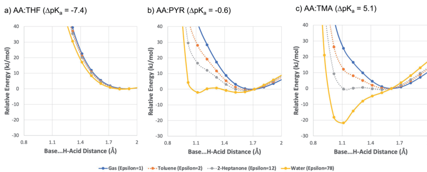
Fig. 5 Computed potential energy curves for the proton transfer reaction (as a function of the H⋯B distance) between the three acid–base pairs in four different solvation environments. The energy is given relative to the most stable neutral acid–base pair configuration. The implicit SMD solvation model is used at the #B97d/6-31+G(d,p) level of theory.
