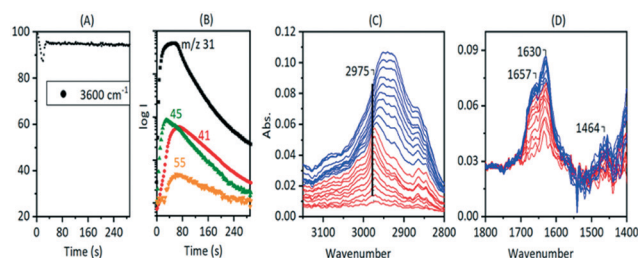
Fig. 15 An 8\text{ }\mu\text{L} pulse of \text{CH}_3\text{OH} at 673 K on HSAPO-34. (A) \nu(\text{OH}) intensity versus time. (B) Corresponding MS traces ( m/z = 31 measures methanol; m/z = 41 , propene with a contribution from fragmentation of DME, m/z = 45 , DME; m/z = 55 , butene). (C and D) Difference infrared spectra at 2 s intervals. Red: from 2 s to 20 s. Blue: from 20 to 40 s.
