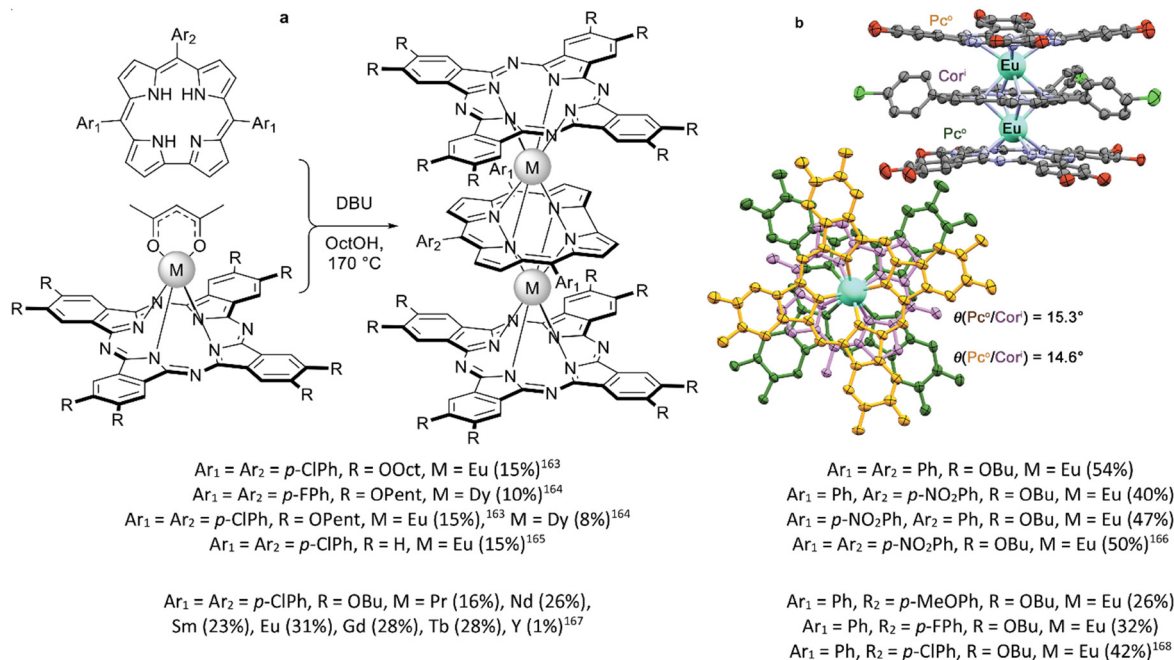
Scheme 30 (a) Synthesis of mixed ligand complexes with phthalocyanine and corrole macrocycles. (b) X-ray structure of the complex \text{Eu}_2[(\text{OAc})_8\text{Pc}]_2[(p\text{-ClPh})_3\text{Cor}] (CCDC HOKQOP). 163 Hydrogen atoms and substituents in top views are not shown for clarity.
