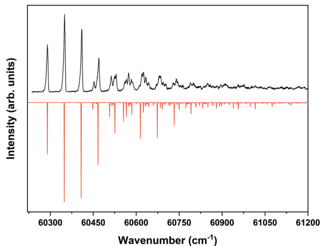
Fig. 4 ZEKE-PFI spectrum obtained for excitation at the S_1 \leftarrow S_0 origin transition ( 31\,059.8\text{ cm}^{-1} ) of the syn/cis conformer of MS together with the corresponding Frank-Condon simulation (red).
