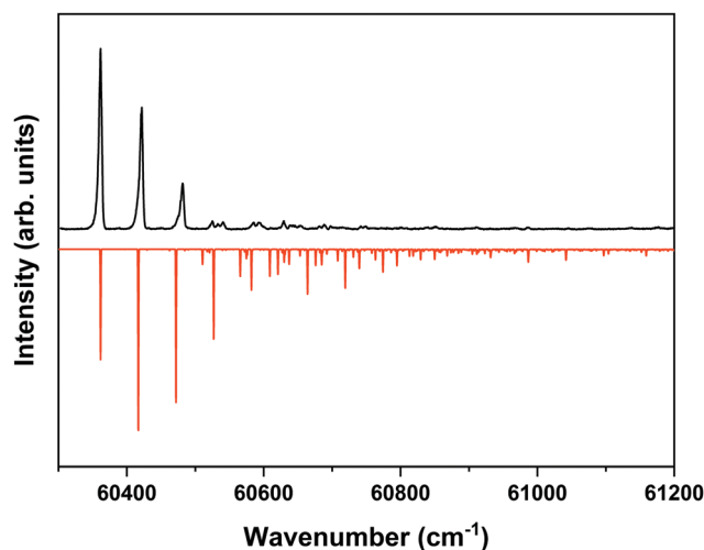
Fig. 5 ZEKE–PFI spectrum obtained for excitation at the S_1 \leftarrow S_0 origin transition ( 31\,170.1 \text{ cm}^{-1} ) of the anti/cis conformer of MS together with the corresponding Franck–Condon simulation (red).
