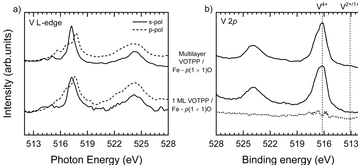
Fig. 5 (a) NEXAFS spectra acquired at the V L_{2,3} -edges and (b) high resolution XPS spectra in the V 2p binding energy range for a single and multilayer VOTPP film on Fe- p(1 \times 1)\text{O} . Spectra acquired with s- (p-)polarized light is presented with full (dashed) lines in panel (a). In panel (b), vertical dashed lines mark the binding energy position of photoemission features from \text{V}^{4+} and \text{V}^{2+/1+} species. 67 The point-by-point difference between the multilayer and the monolayer spectra is reported with a dotted line.
