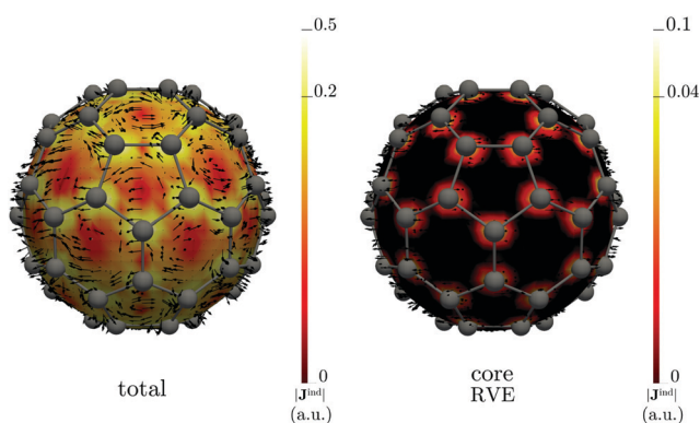
Fig. 6 The J^{\text{ind}} plots of the total current density (left) and the J^{\text{ind}}_{\text{core}} obtained from the RVE approach (right) calculated on the molecular surface of C_{60} . |J^{\text{ind}}| values are given in atomic units ( 1 \text{ a.u.} = 100.63 \text{ nA T}^{-1} \text{ \AA}^{-2} ).
