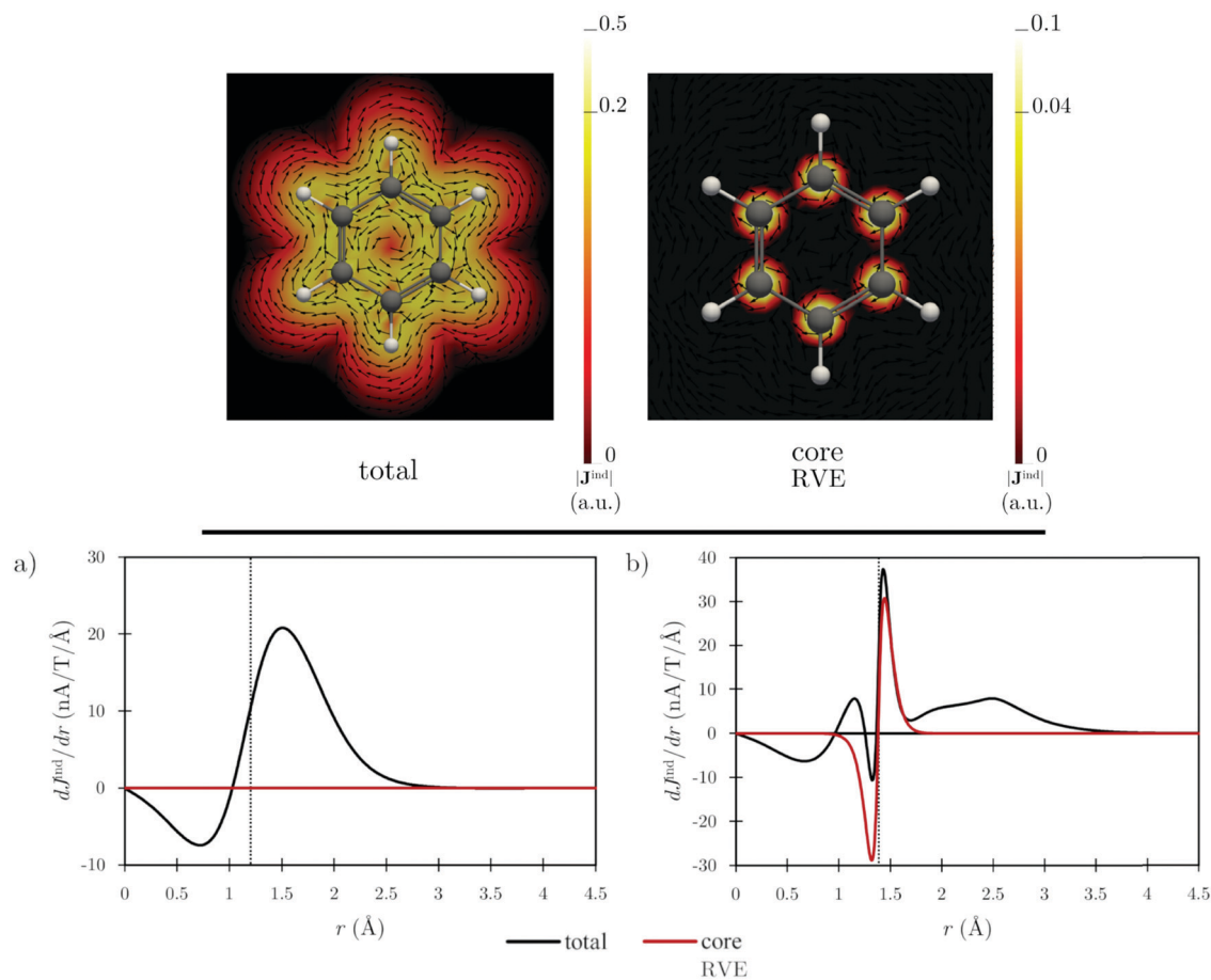
Fig. 2 The top panel shows J^{ind} plots of the total (left) and J^{ind}_{core} obtained from the RVE approach (right) computed in the molecular plane of benzene. |J^{ind}| values are given in atomic units (1 a.u. = 100.63 nA T -1 Å -2 ). The bottom panel shows the dJ^{ind}/dr profiles computed along a plane intersecting: (a) a C–C bond and (b) a carbon and a hydrogen atom of benzene. The vertical dotted lines show the r values corresponding to (a) the C–C bond and to (b) the carbon nucleus, respectively.
