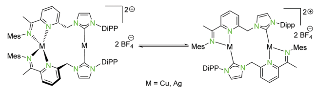
Scheme 5 Isomerisation of homometallic NHC impy ( L 3 ) compounds ( 12 , 14 ) in solution. 43
