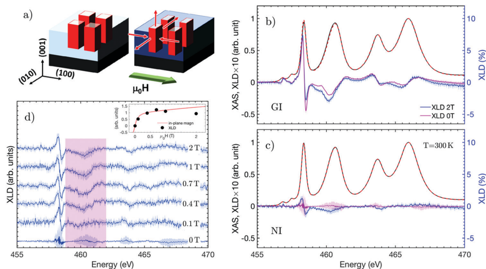
Fig. 3 (a) Schematic showing CFO nanocolumns within the STO matrix (left) and the effect of magnetostriction after applying a magnetic field (right). (b) Ti\ L_{2,3} XAS measured in the grazing incidence (GI) geometry and (c) normal incidence (NI) at 300 K with a 2 T magnetic field applied along the (100) STO axis. The XLD with (blue) and without (pink) the 2 T field are shown for comparison. (d) Room temperature XLD measured in normal incidence geometry at different values of the magnetic field. The pink shading indicates the Ti\ L_3 t_{2g} XLD peak where the strongest spectral changes are observed. In the inset, it can be seen that the dependence of the in-plane magnetization (red) and maximum of the Ti\ L_3 t_{2g} XLD peak (black dots) as a function of the magnetic field agree well.
