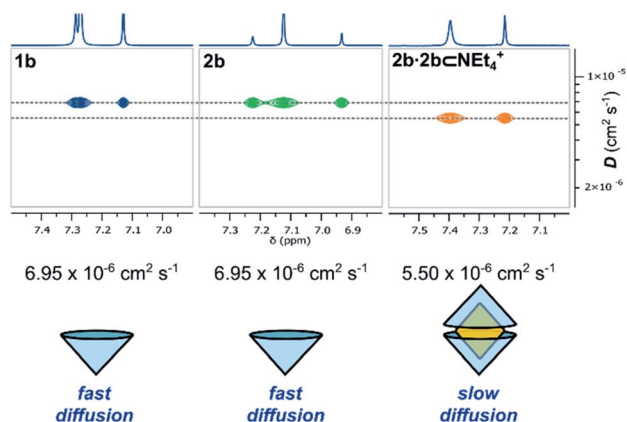
Fig. 4 Truncated ^1\text{H} and DOSY NMR spectra ( d_6 -acetone, 298 K, 500 MHz) of 1b , 2b and 2b·2b·NEt 4 + and their diffusion coefficients.
