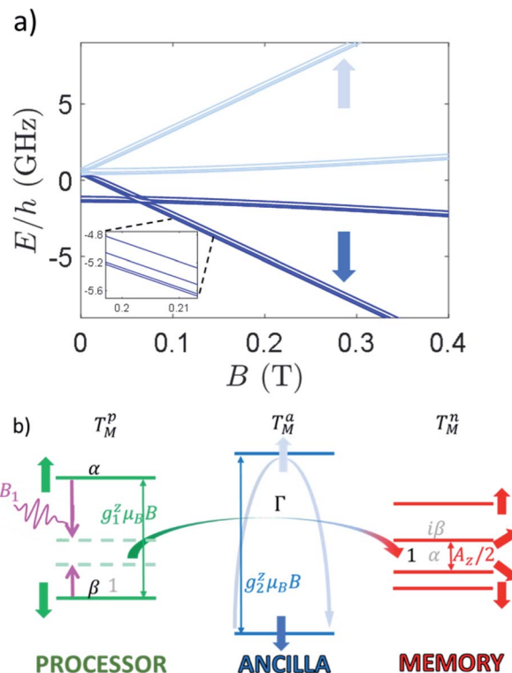
Fig. 5 (a) Zeeman energy level diagram of 2 with a static field applied along z axis. Dark (light) blue levels for B \geq 0.3 T refer to states with the ancilla frozen into its |\downarrow\rangle ( |\uparrow\rangle ) state. Zoom: inset on the low-energy part, highlighting the splitting of nuclear levels induced by hyperfine and quadrupole couplings. (b) Illustrative level diagram of the three units (processor, ancilla and memory), with corresponding energy gaps to first order, in presence of a static field B parallel to z . An oscillating longitudinal field B_1 (purple pulse) is used to compensate the energy mismatch (light green dashed lines) between the processor ( \sim g_1^z \mu_B B ) and the memory ( \sim A_z/2 ), thus inducing an iSWAP gate at a rate T , mediated by a virtual excitation of the ancilla (light blue arrow). The iSWAP transfers an initial superposition of the states of the processor \alpha|-1/2\rangle_1 + \beta|1/2\rangle_1 (with memory in |-1/2\rangle_2 , black coefficients) into a superposition of states of the memory \alpha|-1/2\rangle_2 + i\beta|1/2\rangle_2 (with processor in |-1/2\rangle_1 , grey coefficients).
