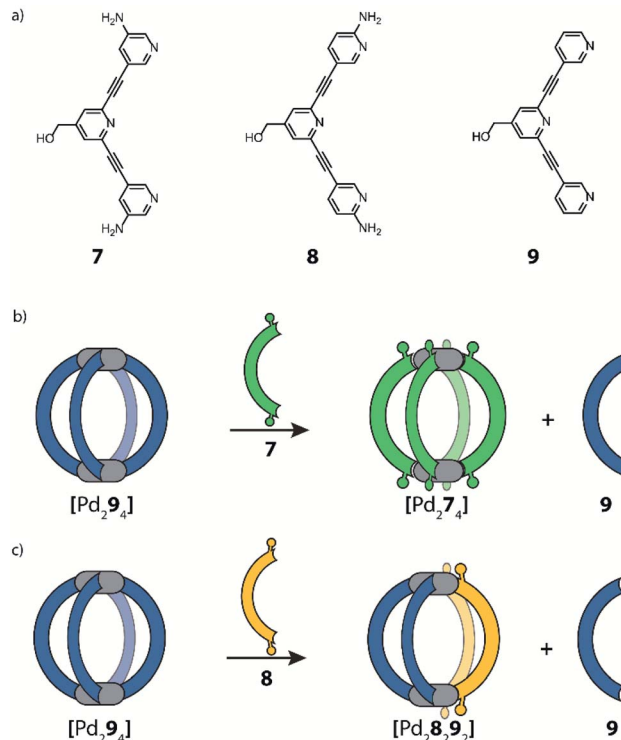
Fig. 6 (a) Banana-shaped ligands bearing amino substituents at the pyridyl donor groups; (b) addition of ligand 7 to [Pd 2 L 9 ] 4 leads to complete displacement of 9 ; (c) formation of heteroleptic cage cis -[Pd 2 L 8.9 ] 2 can be achieved by partial ligand displacement under kinetic control.
