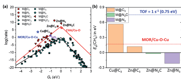
Fig. 6 (a) 1D-volcano plot for methane activation on stable \text{M@N}_x\text{C}_y catalysts. Red and black lines represent scaling lines in \text{CN} = 3 and \text{CN} = 4 , respectively. (b) Calculated E_a(\text{CH}_4) on \text{Cu@C}_3 , \text{Zn@C}_3 , \text{Zn@N}_2\text{C} and \text{Zn@N}_3 . Blue and red lines represent E_a(\text{CH}_4) corresponding to \text{TOF} = 1 \text{ s}^{-1} (0.75 eV) and that on MOR/Cu–O–Cu, respectively. The E_a(\text{CH}_4) of \text{Zn@N}_2\text{C} and \text{Zn@N}_3 is less than 0 eV, since the adsorption of \text{CH}_4 is exothermic and C–H bond dissociation proceeds with almost zero activation energy ( < 0.1 eV).
