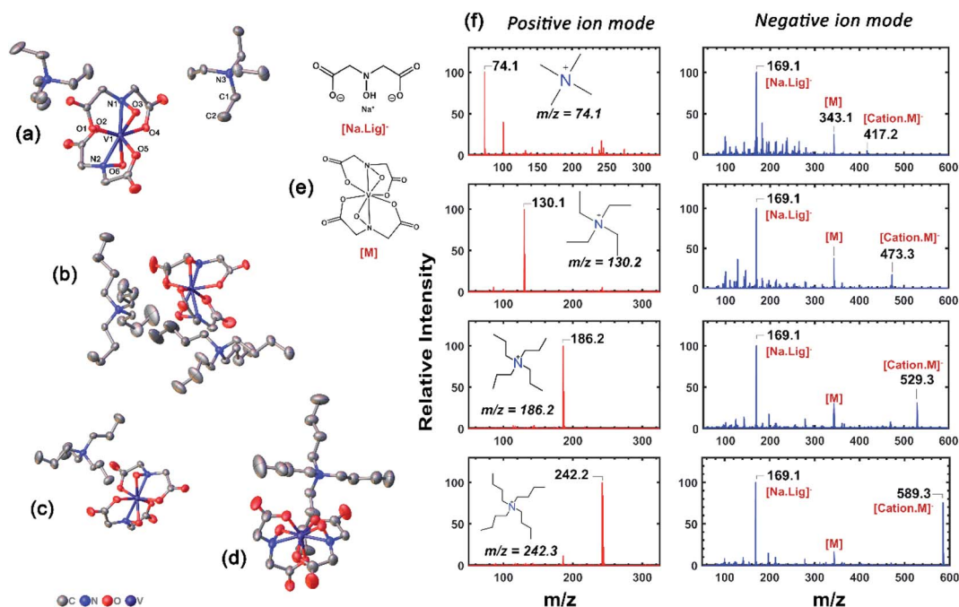
Fig. 4 X-Ray crystallographic data, and mass spectrometric characterization of [\text{N}_{XXXX}]_{1,2}[\text{VBH}] . (a) and (b) correspond to thermal ellipsoid plots of N_{2222} and N_{4444} , bis-alkylammonium, vanadium( 4^+ ) [VBH], respectively and (c) and (d) correspond to those of N_{3333} and N_{4444} mono-alkylammonium, vanadium( 5^+ ) [VBH], respectively. Structures of key ions present in the mass spectrometry are provided in (e) and (f) corresponds to the positive and negative mode mass spectra of [\text{N}_{XXXX}]_2[\text{VBH}] , X = 1 to 4 . Further details of X-ray crystallographic measurements can be found in ESI.†
