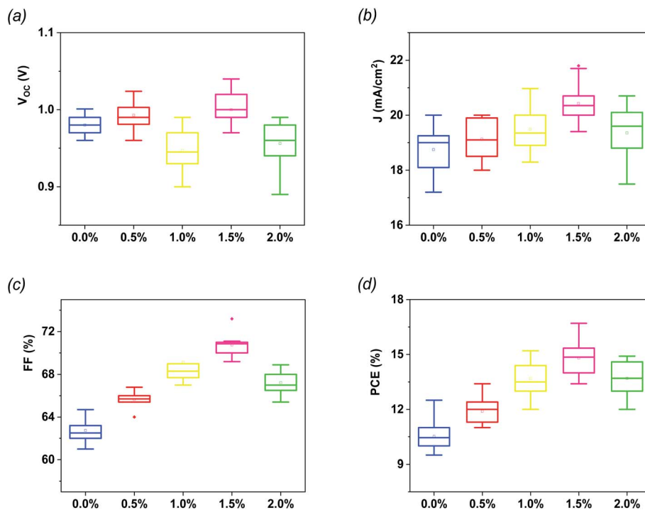
Fig. 2 Statistical histograms of photovoltaic parameters for different PSCs (a) V_{\text{OC}} , (b) J_{\text{sc}} , (c) FF and (d) PCE. Every box shows the parameter distribution of 20 devices.
