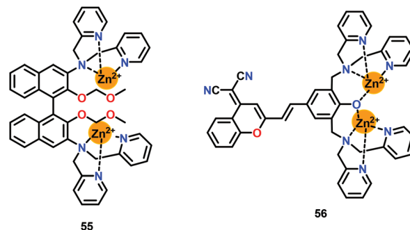
Fig. 27 Chemical drawings of chemosensors 55 and 56. Adapted from ref. 76 and 77.
