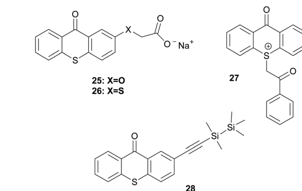
Scheme 7 Examples of initiators bearing the thioxanthone chromophore that work via photodecomposition.
