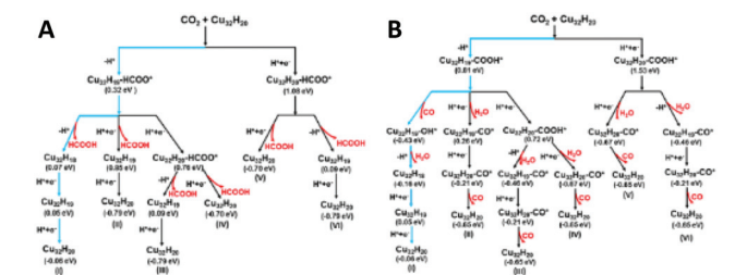
Scheme 9 Theoretical reaction schemes for \text{CO}_2 electroreduction on [\text{Cu}_{32}\text{H}_{20}\{\text{S}_2\text{P}(\text{O}^i\text{Pr})_2\}_{12}] to form (A) \text{HCOOH} and (B) \text{CO} via six different pathways as described in ref. 188 (Reprinted with permission, Copyright 2017 American Chemical Society). The calculated free energy difference ( \Delta G ) for each elementary step is shown under each intermediate state. The most favourable reaction pathway is highlighted in blue.
