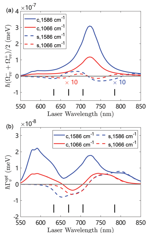
Fig. 5 (a) Vibrational frequency shift (\Omega_{\text{w}}^+ + \Omega_{\text{w}}^-)/2 and (b) effective optomechanical damping rate \Gamma_{\text{w}}^{\text{opt}} = \Gamma_{\text{w}}^- - \Gamma_{\text{w}}^+ as a function of the laser wavelength for the 1586\text{ cm}^{-1} vibrational mode (blue lines) and the 1066\text{ cm}^{-1} vibrational mode (red lines). The solid and dashed lines are the results from the continuum-field model (labeled as “c”) and the single-mode model (labeled as “s”), respectively. The vertical lines indicate wavelengths at 633 nm, 670 nm, 705.9 nm and 785 nm used for later simulations. The laser intensity is 1\text{ }\mu\text{W }\mu\text{m}^{-2} and other parameters are specified in the text.
