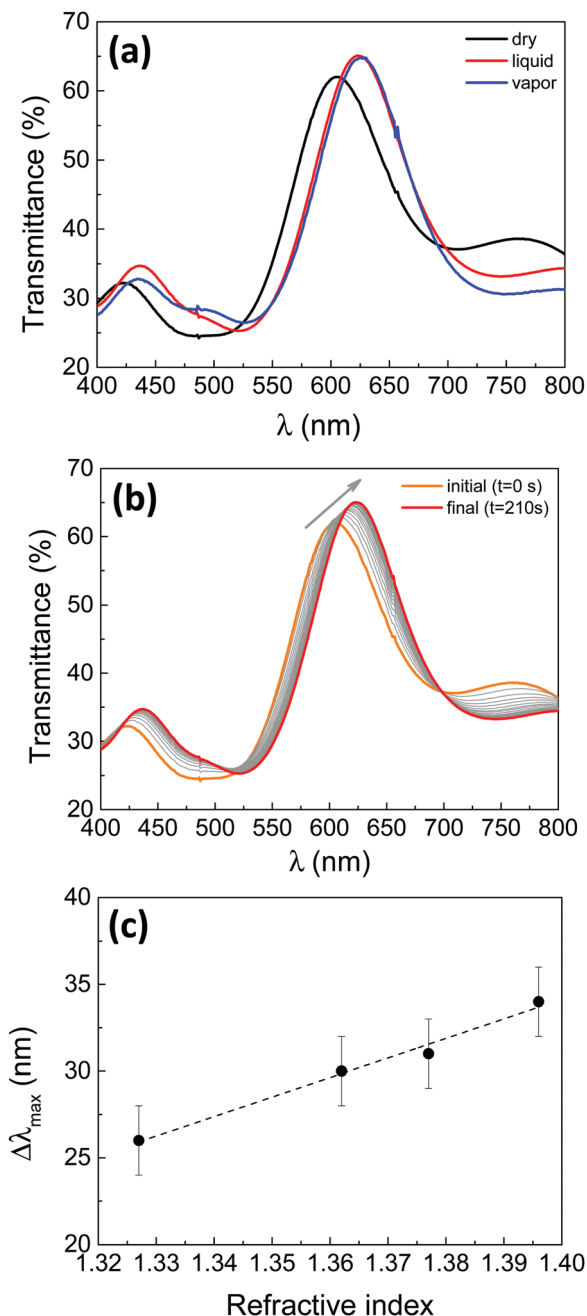
Fig. 6 (a) UV-Visible spectra of 4\times(\text{SC}/\text{TF})/\text{Au}/\text{TSV} measured dry, in an atmosphere saturated with butanol vapour and after immersion in liquid butanol. (b) UV-visible spectra of the same device as a function of time in contact with liquid butanol. The orange curve corresponds to the initial state (dry, t = 0 s) and the red one to the final state (full of solvent, t = 210 s). (c) Linear calibration curve for the variation of the Tamm plasmon peak position of the protected device as a function of refractive index for different vapours (alcohols) filling the pores.
