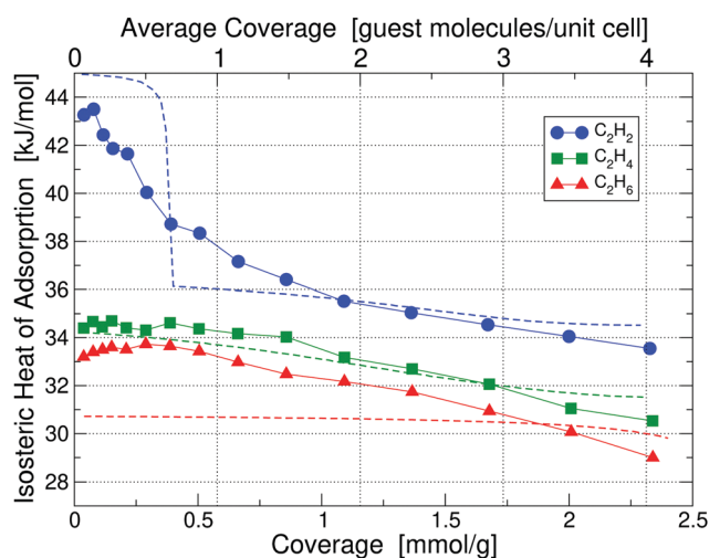
Fig. 6 Isothermic heats of adsorption of C 2 H 2 , C 2 H 4 and C 2 H 6 in UiO-66(Zr)-NO 2 at 195 K, obtained by calorimetry measurements; results for 293 K are shown in Fig. S6 (ESI†). Dashed lines correspond to our partition-function occupancy-probability calculations based on our theoretical binding energies and availability of binding sites.
