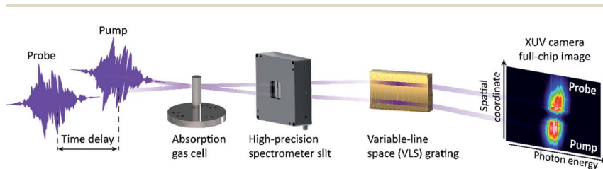
Fig. 1 Measurement principle of split-beam XUV-pump XUV-probe transient-absorption spectroscopy. After focusing the pulses into the absorption gas cell filled with a moderately dense gas medium the transmitted pulses are coupled into a grating spectrometer consisting of a high precision slit, a VLS grating, and an XUV-sensitive camera which simultaneously detects the spatially separated pump and probe pulse spectra on a single-shot basis.
