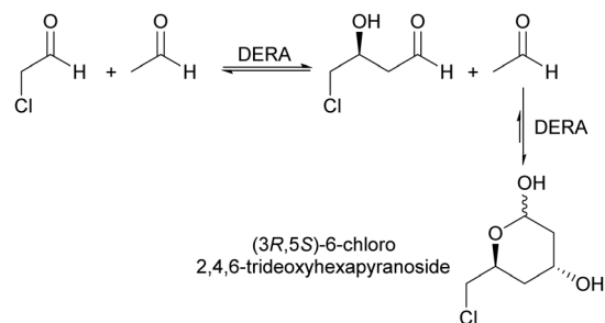
Scheme 1 Sequential aldol condensation catalysed by DERA for the synthesis of a chiral statin precursor.
