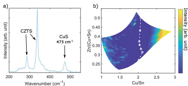
Fig. 2 (a) Raman spectrum (532 nm excitation) with CZTS Raman modes in the range 250–400 \text{cm}^{-1} . CuS mode visible at 475\text{ cm}^{-1} . (b) Integrated intensity in the region of the CuS peak against the cation composition from EDX. The phase boundary for CuS is marked with a white dashed line.
